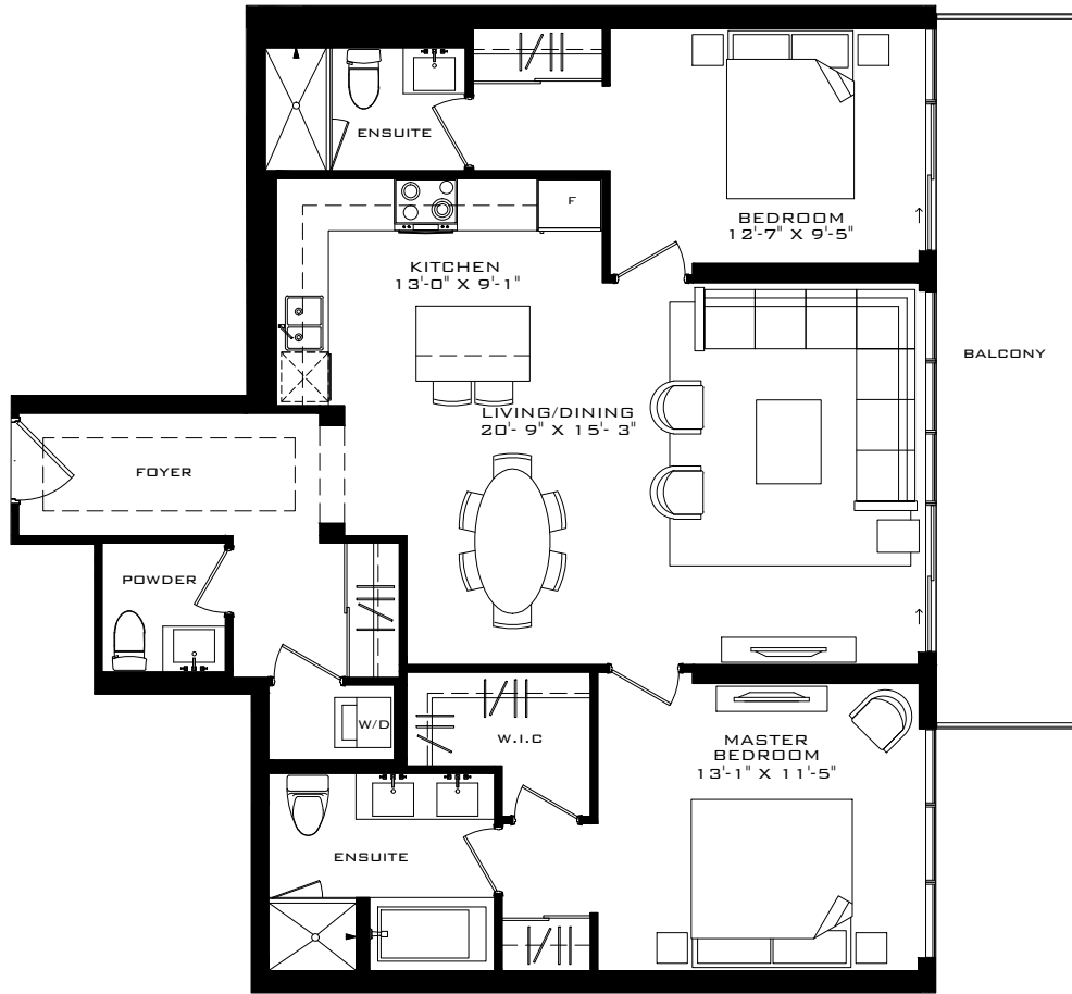
SUITE 11 2 BEDROOM 1160 sq. ft.
